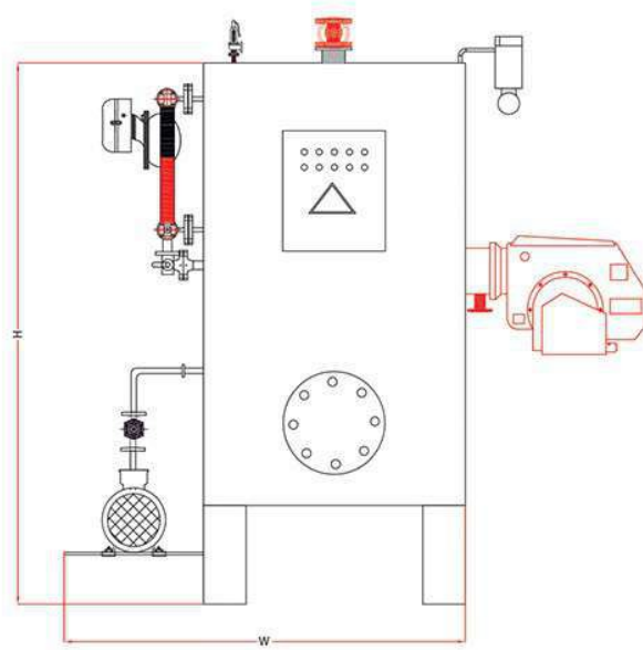
Technical Table Vertical Steam Boiler
